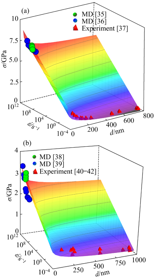
Fig. 4 Comprehensive effects of size and strain rate on yield strengths of monocrystalline copper (a) and gold (b) nanowires
