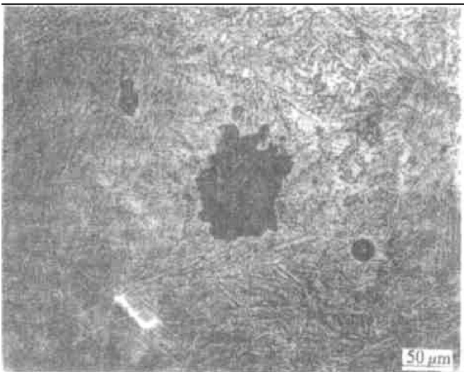
Fig. 3 Morphology of sample 5AS1N after pitting (WM, 65 °C, 2 min)
