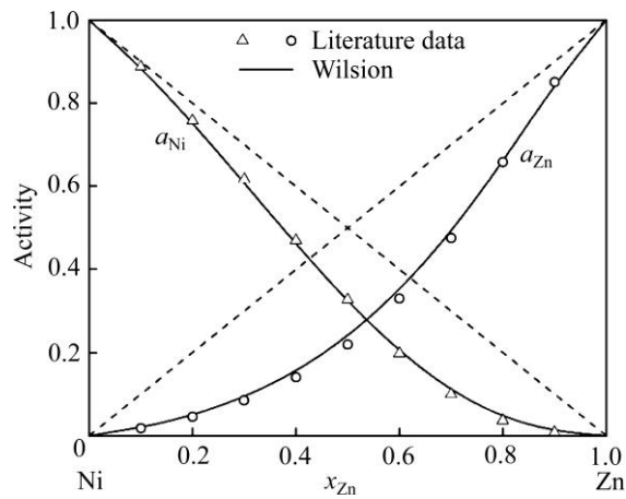
图 1 Zn-Ni 合金组元活度 Wilson 方程计算值与实验值对比 Fig. 1 Comparison between calculated and experimental values of activity of Zn-Ni alloy components by Wilson equation
