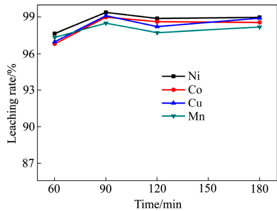
图 4 还原时间对有价值金属浸出率的影响 Fig. 4 Effect of reduction time on leaching rate of valuable metals
