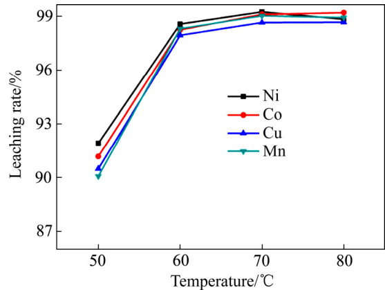
图 7 浸出温度对有价金属浸出率的影响 Fig. 7 Effect of leaching temperature on leaching rate of valuable metals
