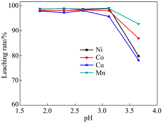
图 6 浸出 pH 对有价值金属浸出率的影响 Fig. 6 Effect of leaching pH on leaching rate of valuable metals
