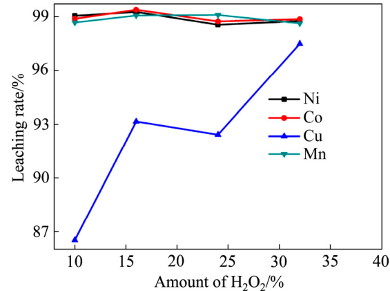
图 8 双氧水加入量对有价金属浸出率的影响 Fig. 8 Effect of amount of H 2 O 2 on leaching rate of valuable metals
