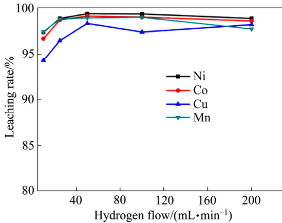
图 5 氢气流量对有价值金属浸出率的影响 Fig. 5 Effect of hydrogen flow on leaching rate of valuable metals
