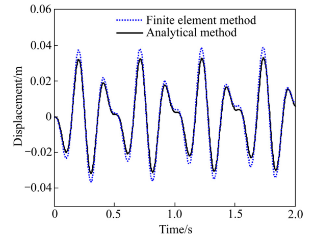
图 3 本文算法与解析法求解结果对比 Fig. 3 Comparison between finite element method and analytical method
