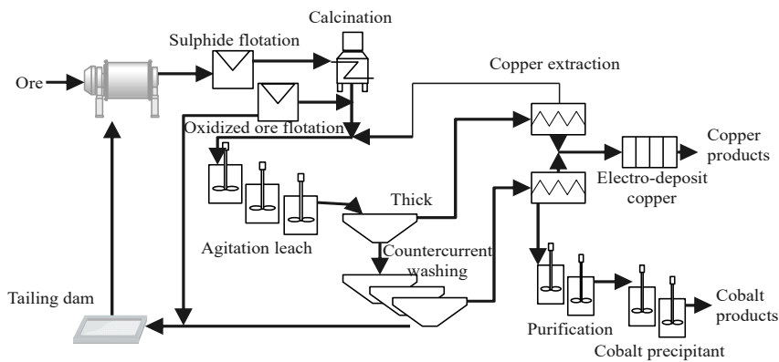
图 6 硫化矿-氧化矿分步浮选-焙烧-浸出联合流程 Fig. 6 Combined process of step flotation - roasting - leaching of oxidized-sulfide ore.
