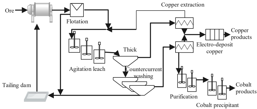
图 5 硫化浮选—湿法浸出联合流程 Fig. 5 Combined process of sulfidized flotation and hydro-leaching.
