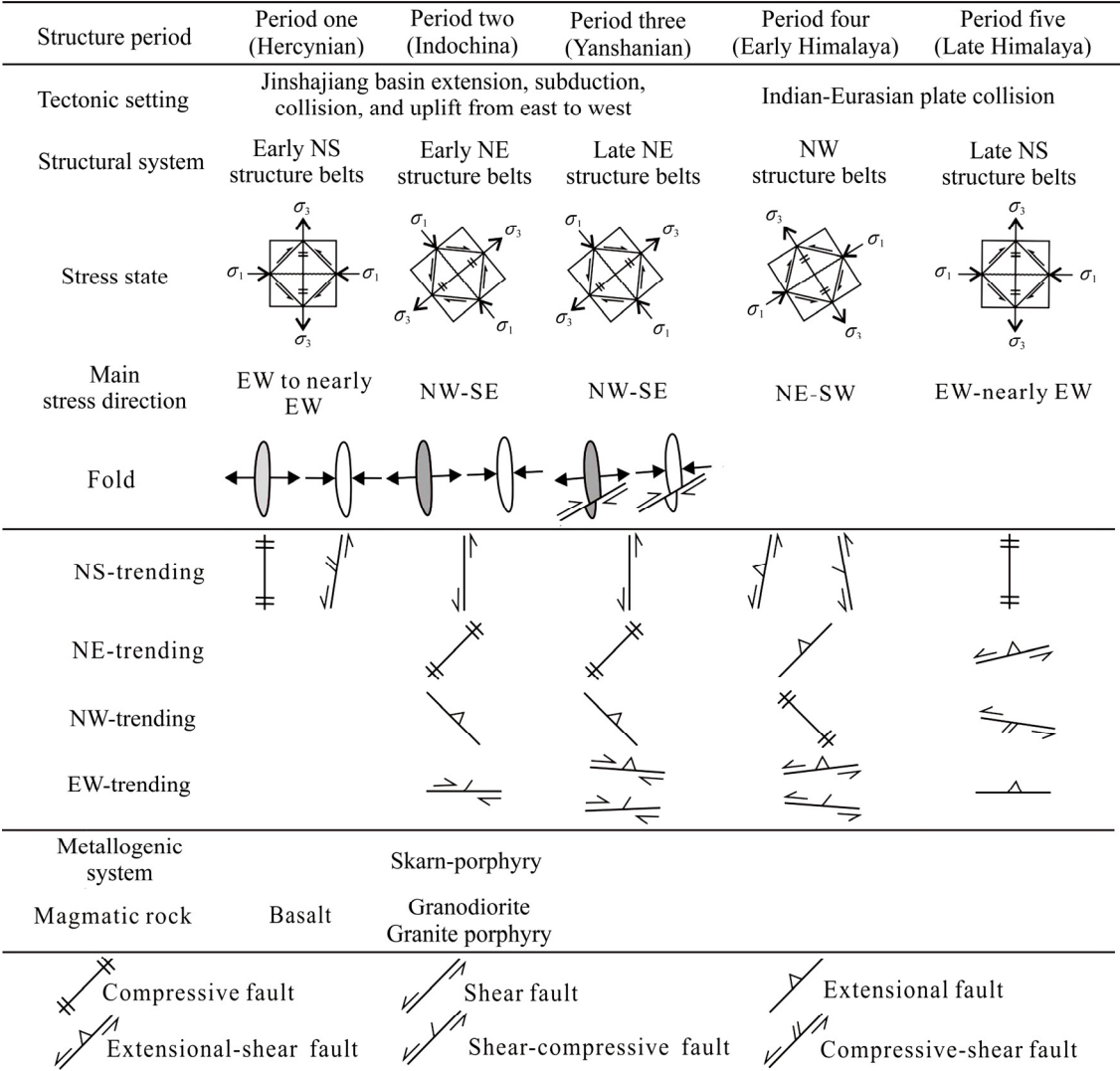
图 8 羊拉铜矿床断裂体系示意图(地质年代划分据文献[34]) Fig. 8 Ore-field structural system of Yangla Cu deposit (Age of geology from Ref. [34])
