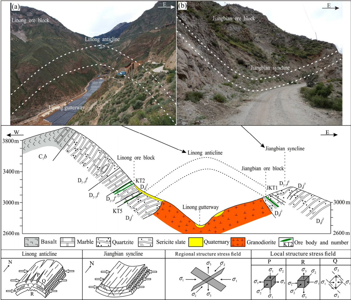
图 3 羊拉铜矿床褶皱应力分析示意图(剖面图据文献[5, 16]; 力学性质分析据文献[13]修改) Fig. 3 Fold stress analysis of Yangla Cu deposit (Geological section from Refs. [5, 16] and mechanical property from Ref. [13]): \sigma_1 —Maximum compressive stress; \sigma_2 —Moderate compressive stress; \sigma_3 —Minor compressive stress
