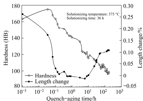
Fig. 7 Hardness and length change versus quench-aging time curves of Zn-40Al-2Cu-2Si alloy obtained at 180 °C
