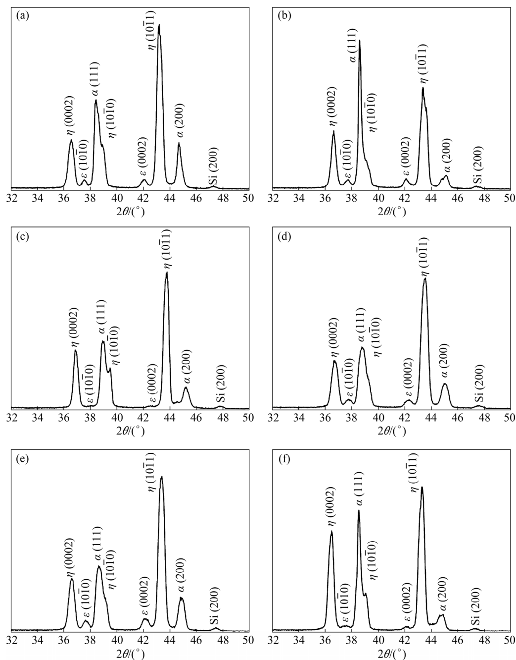
Fig. 4 XRD patterns showing phases in as-cast (a), and H1 (b), H2 (c), T5 (d), T6 (e) and T7 (f) heat-treated microstructures of Zn-40Al-2Cu-2Si alloy
