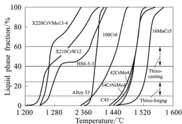
Fig.3 Liquid fraction behavior vs temperature for different steels using DTA at heating rate of 10 °C/min[29]
