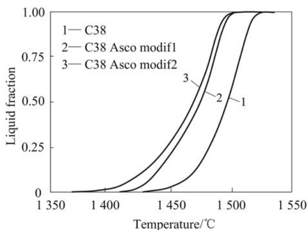
Fig.2 Liquid fraction behavior vs temperature and comparison between classical C38 steel grade and modified one
