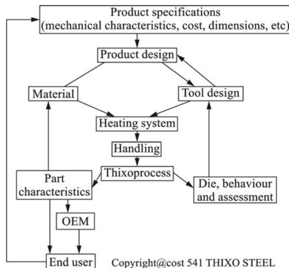
Fig.1 Thixoforming of steels, conception and realization diagram
