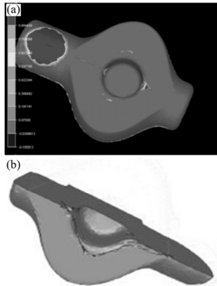
Fig.4 Material flow modelling (a) and real part (b) showing defects around central air intake hole
