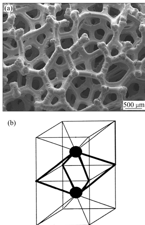
图1 网状多孔金属材料实际孔隙形貌及简化结构模型 Fig. 1 Real pore morphology of reticulated porous metallic materials and simplified structure model: (a) Pore morphology of representative metal foam; (b) Pore unit of octahedral structure model
