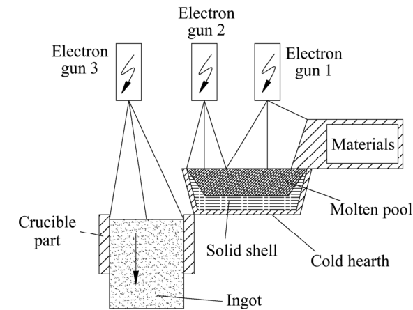
图 1 EB 炉熔炼区域及各电子枪扫描区域示意图 Fig. 1 Diagram of melting area and scanning area of electron gun of EB furnace
