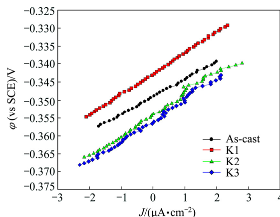
Fig. 3 Linear polarization curves for CuAlNi alloy in 0.9% NaCl solution
