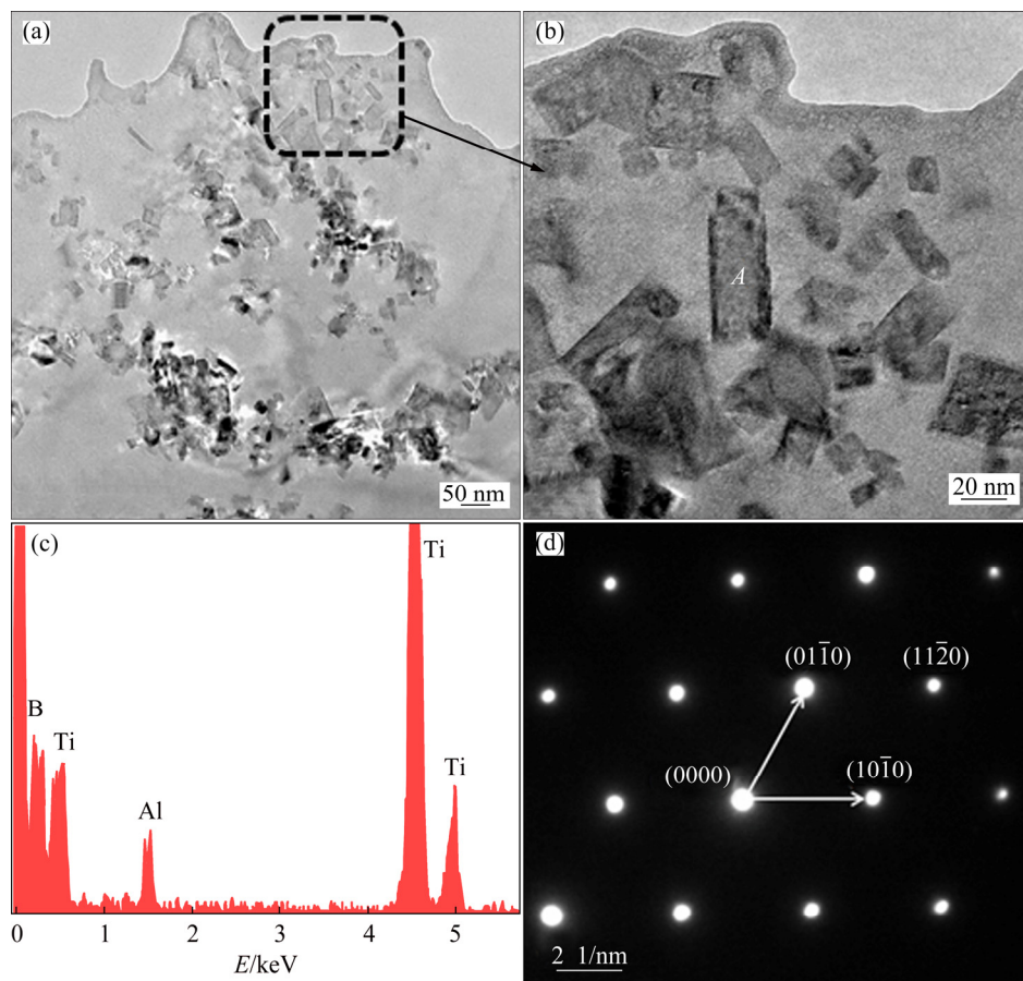
Fig. 3 TEM images (a, b), EDS result (c) and SADP (d) of \text{TiB}_2 nanoparticles in as-cast Alloy T30
