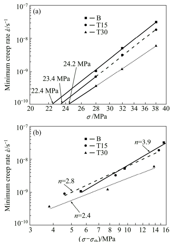
Fig. 7 Threshold stress \sigma_{\text{th}} (a) and true stress exponent n (b) of alloy after heat treatment at 375 ^{\circ}\text{C} for 48 h
