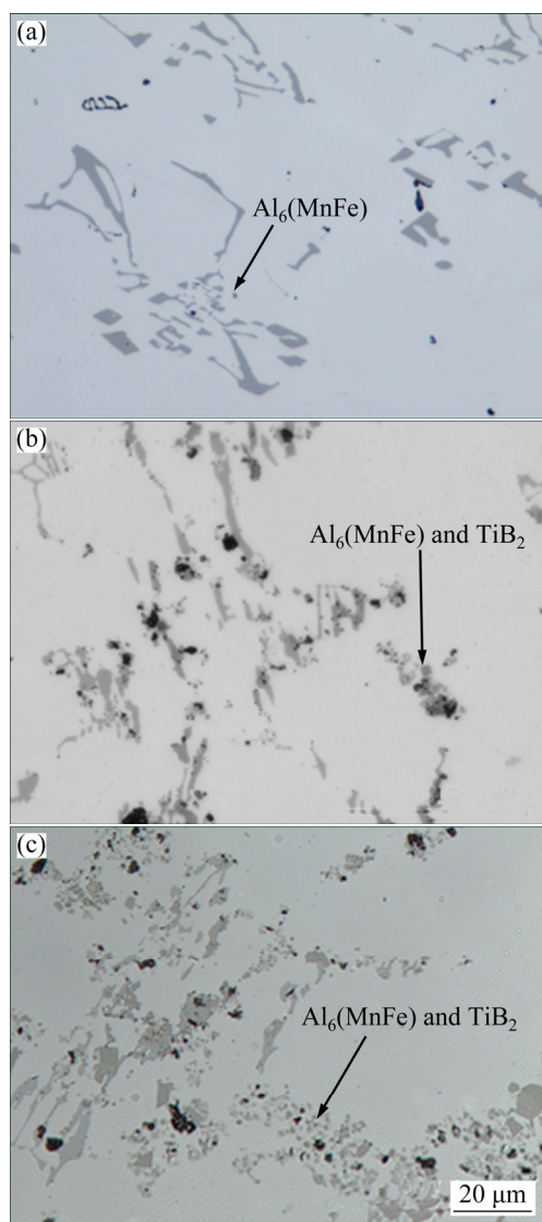
Fig. 1 Microstructures of as-cast Alloy B (a), Alloy T15 (b) and Alloy T30 (c)
