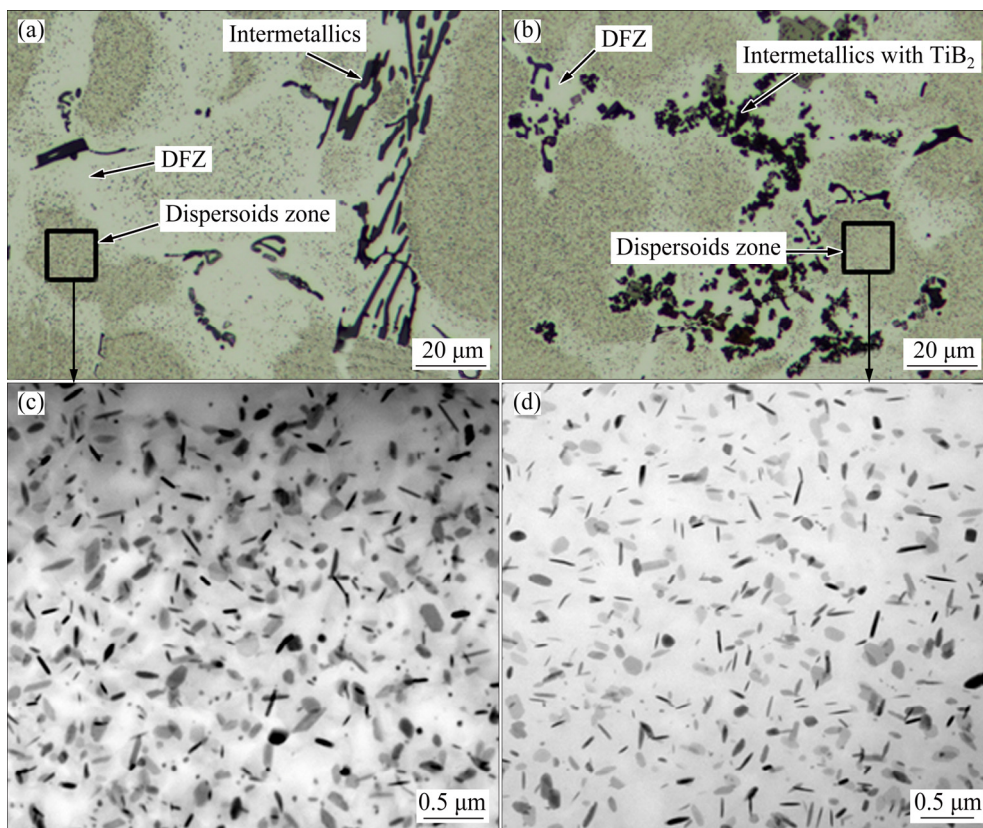
Fig. 4 Distribution of dispersoids and DFZ in Alloy B (a, c) and Alloy T30 (b, d) after heat treatment at 375 °C for 48 h
