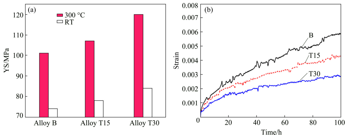
Fig. 5 YS of alloy at both RT and 300 °C (a) and creep curves of alloy at 300 °C (b) after heat treatment at 375 °C for 48 h
