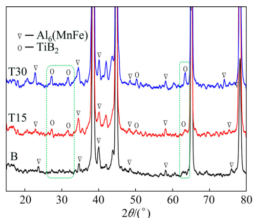
Fig. 2 XRD patterns of experimental alloys in as-cast condition
