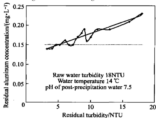
Fig. 2 Relativity between residual turbidity and residual aluminum concentration of post-precipitation
