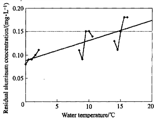
Fig. 3 Influence of water temperature on residual aluminum concentration (pH value of post-precipitation: 7.5)
