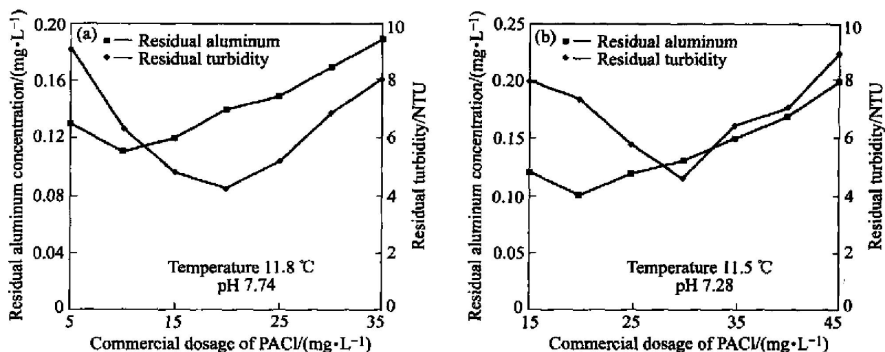
Fig. 1 Influence of coagulant dosage on residual turbidity and residual aluminum concentration (a) —Raw water turbidity 35 NTU; (b) —Raw water turbidity 105 NTU
