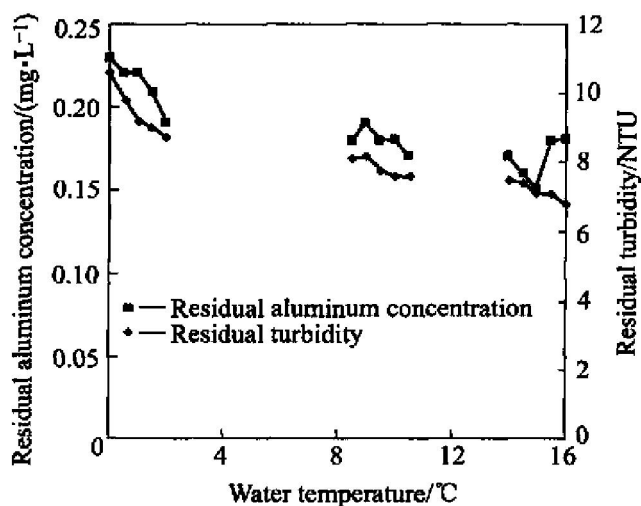
Fig. 4 Average values of residual aluminum and residual turbidity of post-precipitation water
