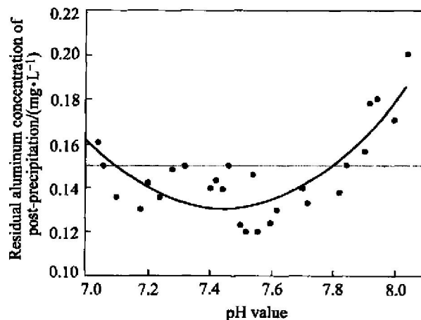
Fig. 5 Correlation of pH value and residual aluminum (Turbidity of raw water 80 NTU; temperature 14 °C)
