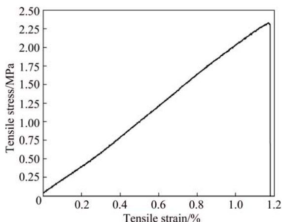
Fig. 6 Tensile stress–strain curve of \text{Ni}_{68.6}\text{W}_{17.9}\text{B}_{13.5} amorphous ribbons
