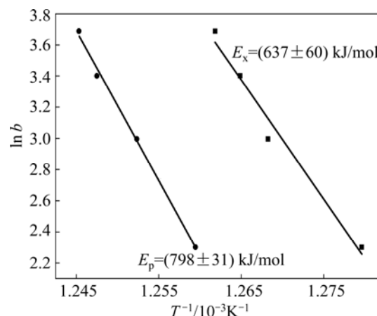
Fig. 5 Ozawa plot for \text{Ni}_{68.6}\text{W}_{17.9}\text{B}_{13.5} amorphous ribbons
