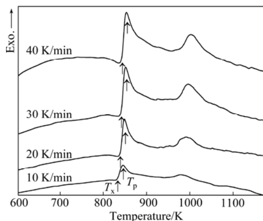
Fig. 4 DSC curves of \text{Ni}_{68.6}\text{W}_{17.9}\text{B}_{13.5} amorphous ribbons under different heating rates
