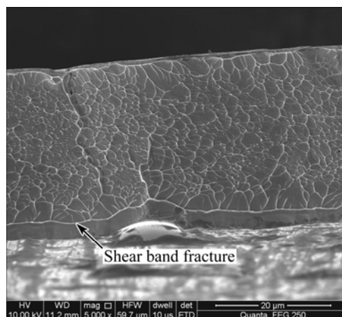
Fig. 7 SEM image of fracture of \text{Ni}_{68.6}\text{W}_{17.9}\text{B}_{13.5} amorphous ribbons
