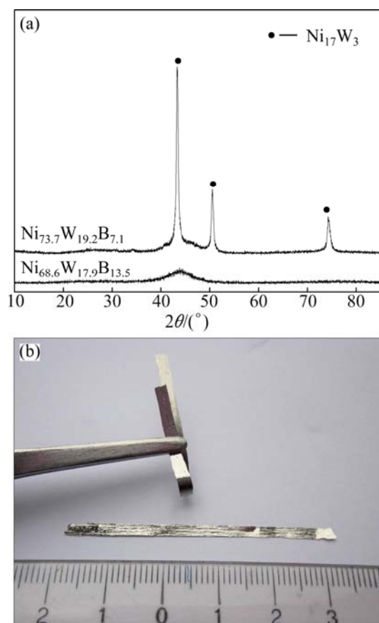
Fig. 1 XRD patterns of as-prepared \text{Ni}_{73.7}\text{W}_{19.2}\text{B}_{7.1} and \text{Ni}_{68.6}\text{W}_{17.9}\text{B}_{13.5} ribbons (a) and optical image of \text{Ni}_{68.6}\text{W}_{17.9}\text{B}_{13.5} ribbons (b)
