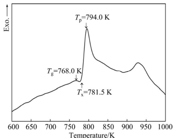
Fig. 3 DSC curve of \text{Ni}_{68.6}\text{W}_{17.9}\text{B}_{13.5} amorphous ribbons
