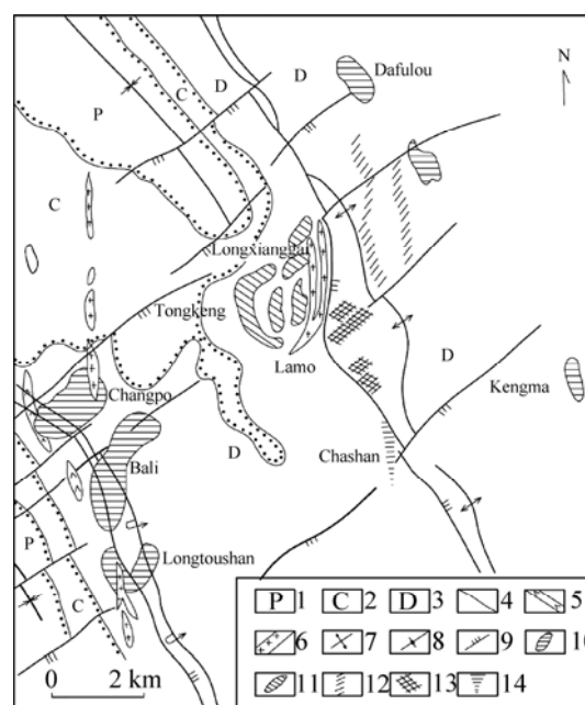
Fig. 1 Mineralization zoning of Dachang ore field (compiled from China Nonferrous Metals Industry Corporation, 1987): 1 — Permian limestone and siliceous; 2 — Carboniferous limestone; 3—Devonian limestone, shale and siliceous; 4—Parallel unconformity stratigraphic contact; 5 — Diorite porphyrite; 6—Granite and granite porphyry; 7—Anticline axis; 8—Syncline axis; 9—Faults; 10—Tin ore; 11—Zn–Cu ore; 12—Scheelite veins; 13—Wolframite veins; 14—Antimony veins
